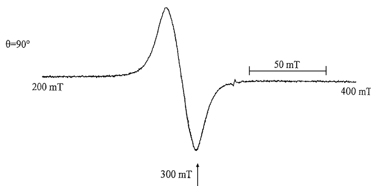
Figure 2. Single crystal X-band EPR spectrum of the nickel complex at room temperature in the ab plane. The EPR spectrum corresponds to the orientation when the applied magnetic field ( B ) is parallel to the crystal b -axis. Frequency = 9.09134 GHz.
