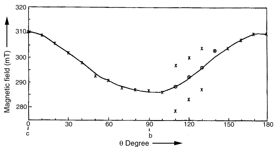
Figure 7. Isofrequency plot in the bc plane for nickel(II)/Hsalamp complex at room temperature. Frequency = 9.09248 GHz.
